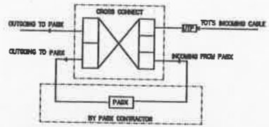
TELEPHONE SYSTEM SCHEMATIC
