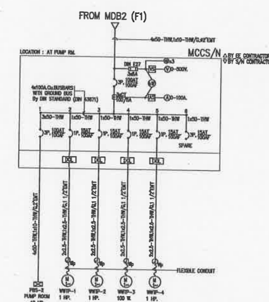
SINGLE LINE DIAGRAM FOR MCCS/N
