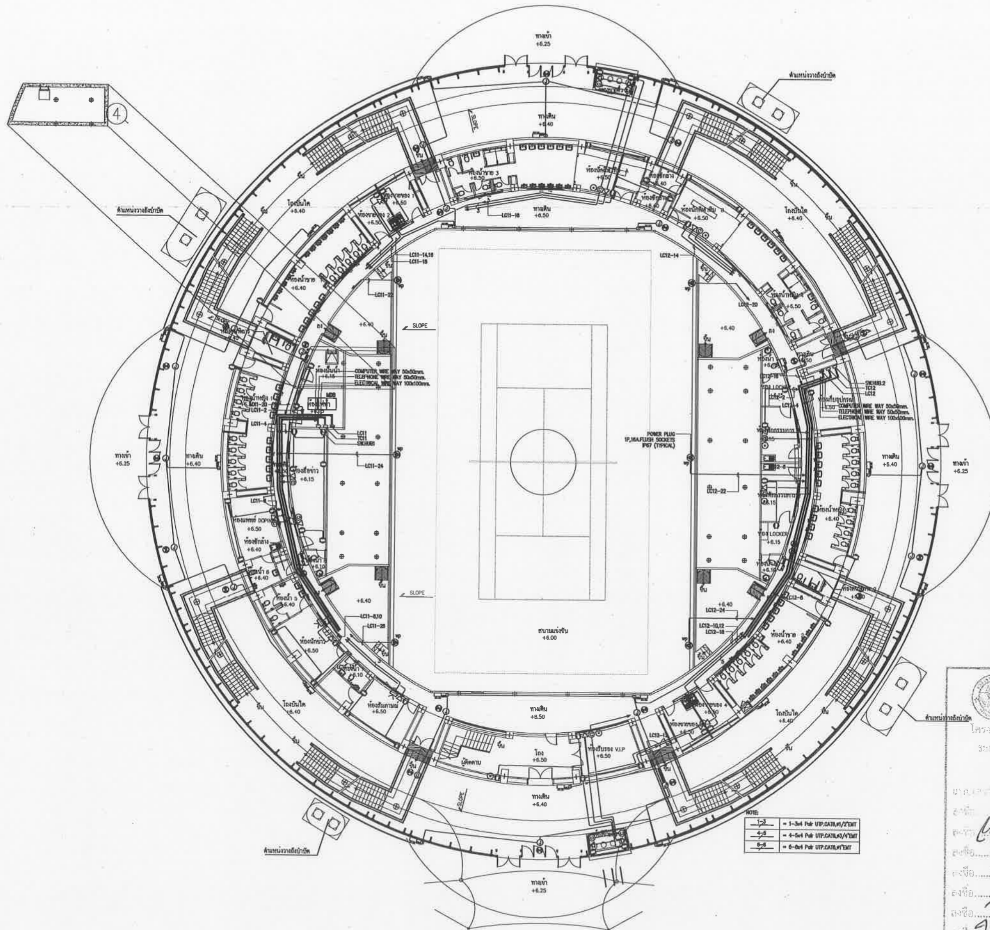
RECEPTACLE, TELEPHONE, COMPUTER, MATV OUTLET & EMERGENCY LIGHT 1st PLAN
