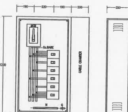
FACE LAYOUT FOR MCCS/N
