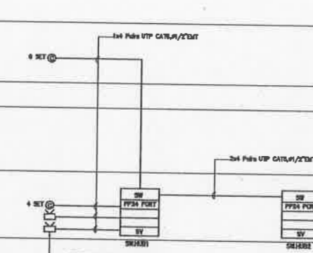
COMPUTER SYSTEM RISER DIAGRAM
