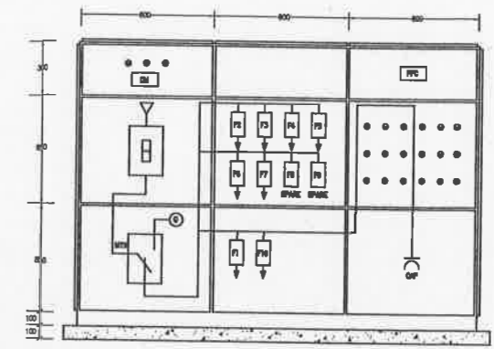
FACE LAYOUT FOR MDB2
