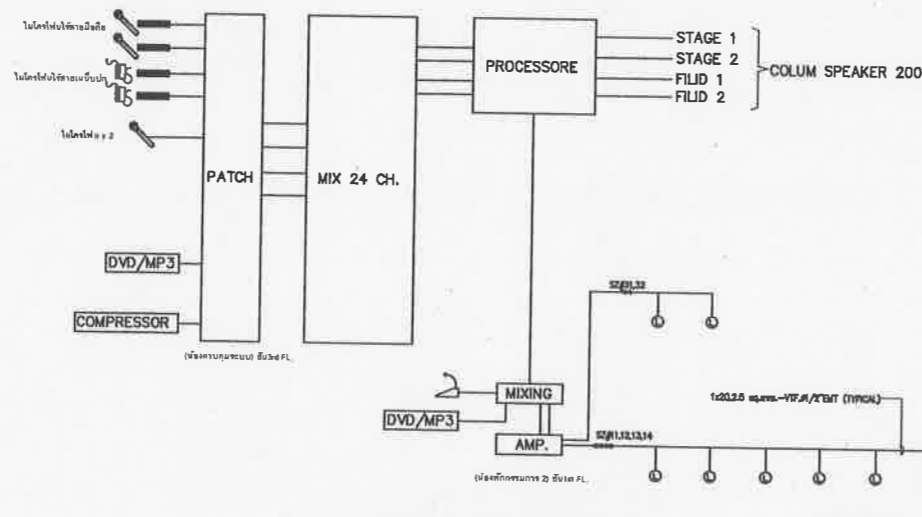
SOUND SYSTEM RISER DIAGRAM
