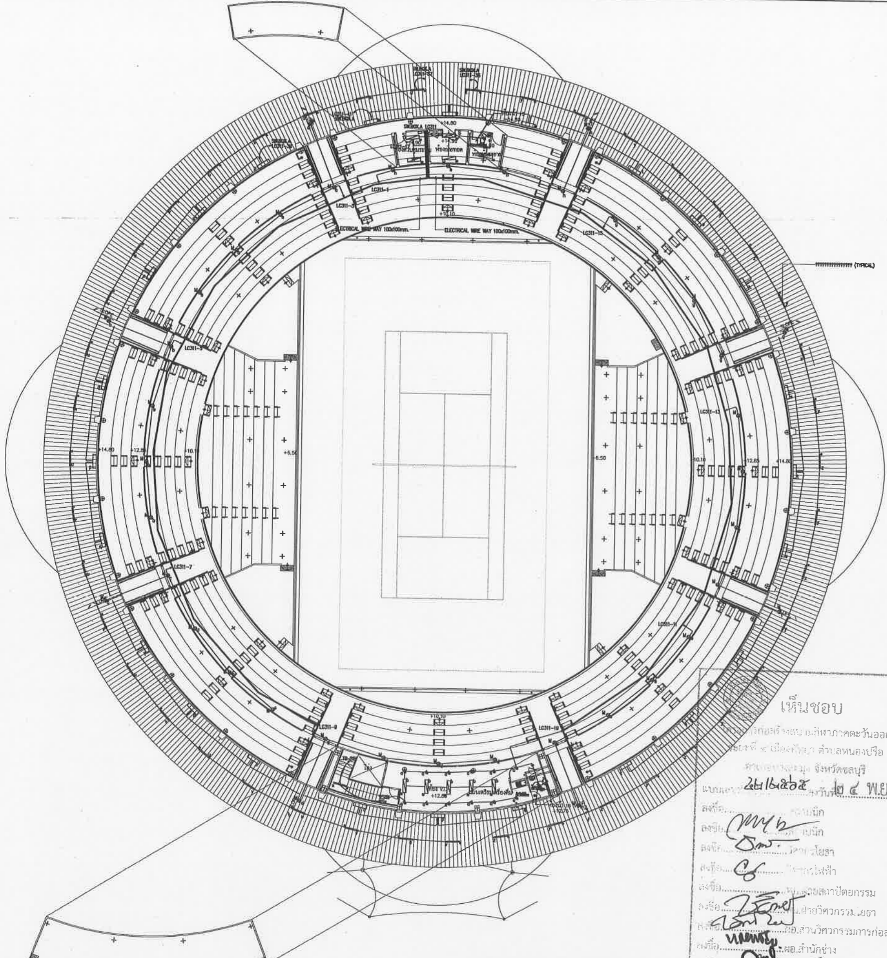
LIGHTING FIXTURE LAYOUT 3rd PLAN
