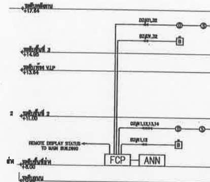
FIRE ALARM SYSTEM RISER DIAGRAM
