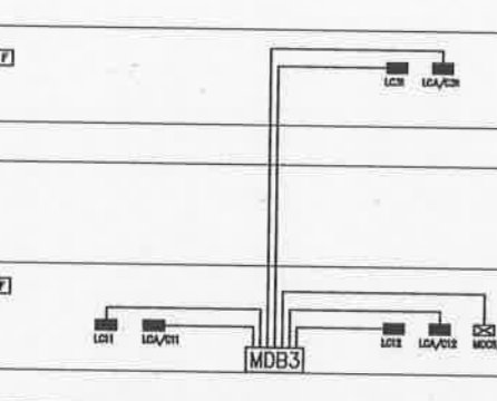
ELECTRICAL POWER SYSTEM RISER DIAGRAM
