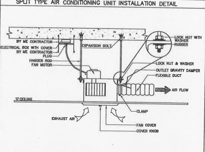
CEILING MOUNTED CASSETTE FAN DETAIL.
