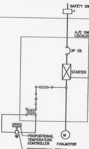
FOR AHU
